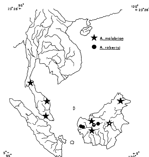
Fig. 9. Known distribution of Acanthopsoides molobrion and A. robertsi . Open symbols represent the type locality; symbols represent physical locals, not necessarily number of individual collections.
