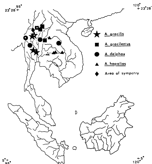
Fig. 4. Known distribution of Acanthopsoides gracilis , A. gracilentus , A. delphax , and A. hapalias . Open symbols represent the type locality; symbols represent physical locals, not necessarily number of individual collections.
