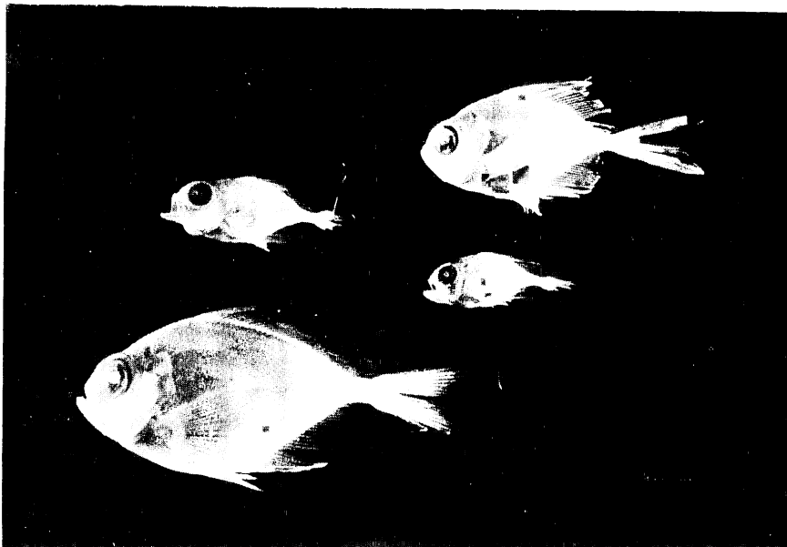
Fig. 2. Juvenile Brama japonica from the Southeast Hancock Seamount: 15.1, 19.5, 26.0, and 38.6 mm SL.
